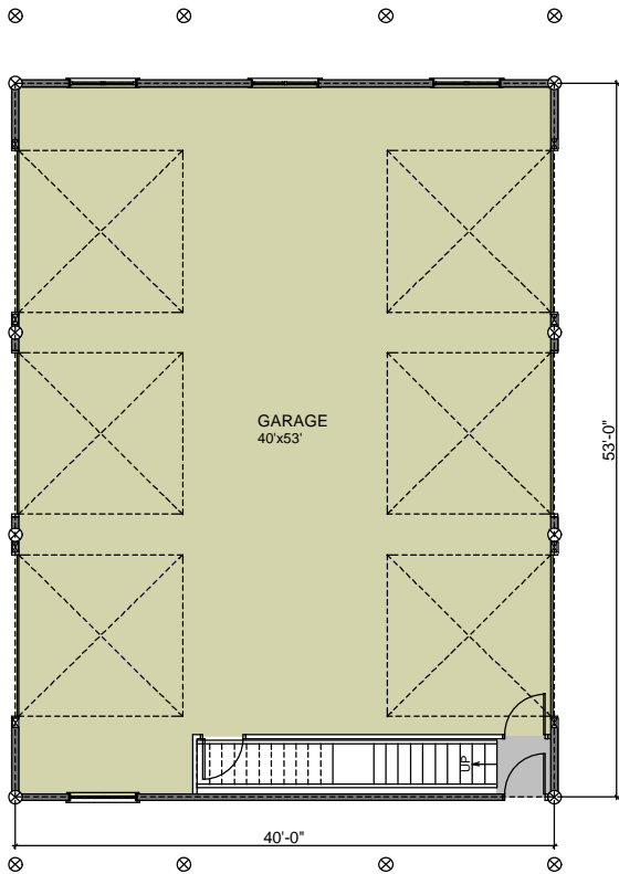
GARAGE FIRST FLOOR PLAN AREA: 2167 SQ.FT.
